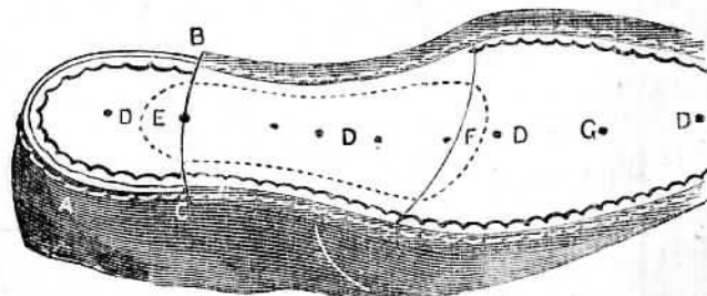
Fig. 93.—Welt Sewn in.
