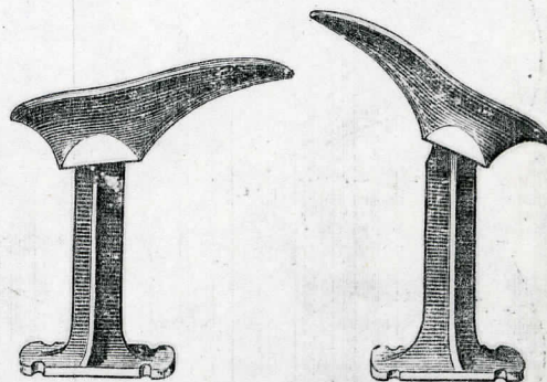
Figs. 19, 20.—Last Stands, with Reversible Foot.
