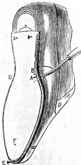
Fig. 99.—Stitching the Boot.
