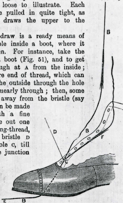
Fig. 51.—Stitch Drawing.
