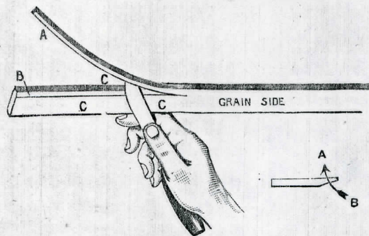
Fig. 53.—Cutting Welts.
