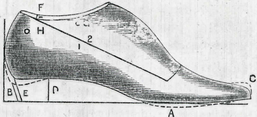
Fig. 68.—A Last.
