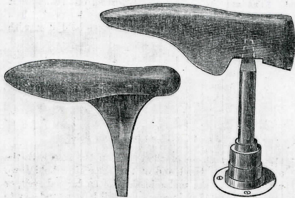
Fig. 18.—Iron Last and Stand.
